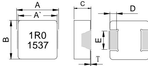
non-leadframe
