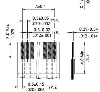
Accommodated FFC/FPC
