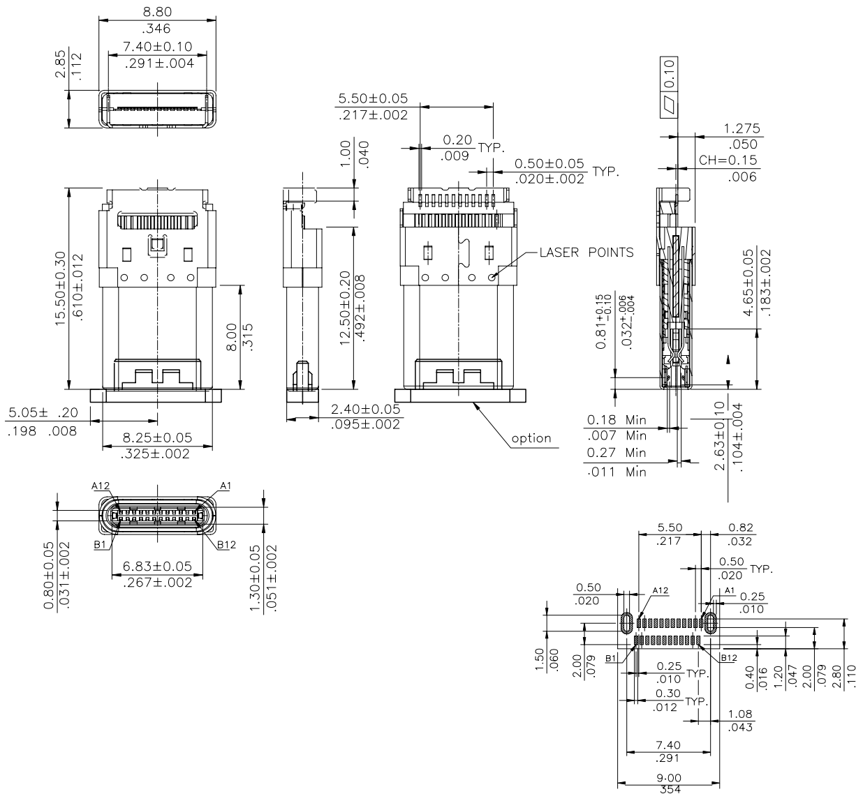
RECOMMENDED P.C.B. LAYOUT (T:1.00mm or 0.80mm) TOLERANCE ±0.05mm
