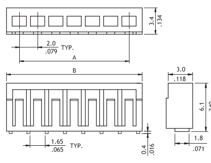
P/N CI02T021*E0
