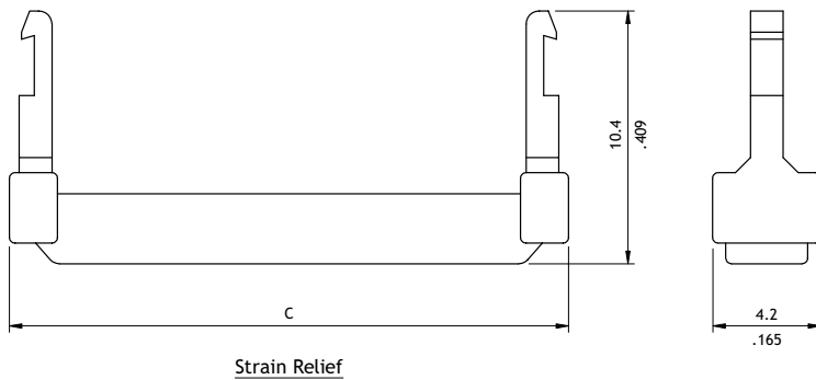
Strain Relief
