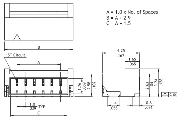
P/N CI14**M1HRE-NH
