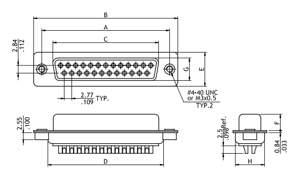
Receptacle Connector(K0/K1Type)
