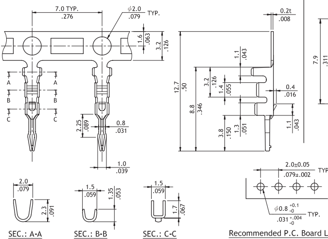
P/N CI02T011*E0
