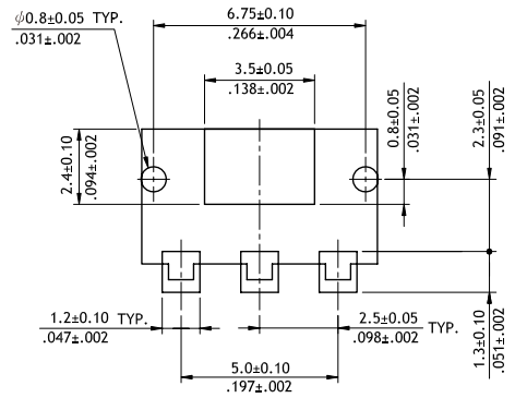
Recommended P.C Board Layout Thickness: 0.80mm
