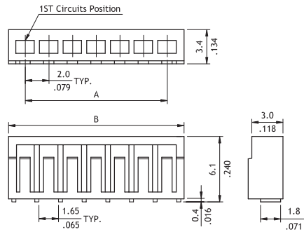
P/N CI02T011*E0
