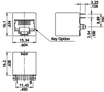
8 Positions
