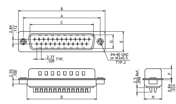
Plug Connector(K0/K1Type)
