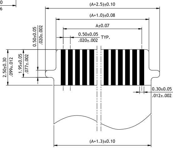
Accommodated FFC/FPC
