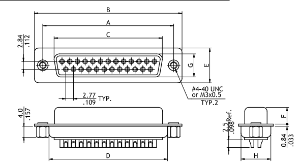
Receptacle Connector(C0/C1Type)
