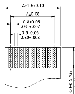
Accommodated FFC/FPC (Thickness: 0.3 ± 0.03)
