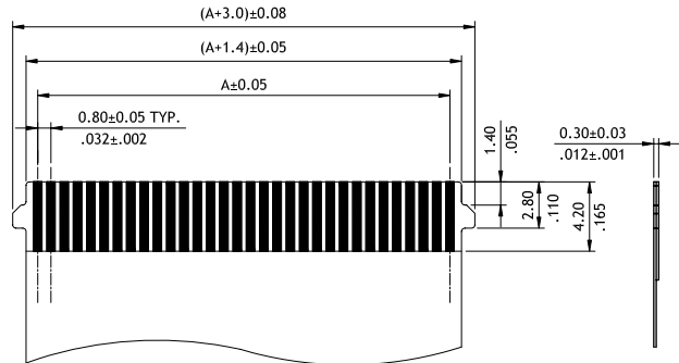
Accommodated FFC/FPC
