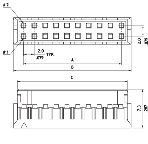
With Locking Ramp
