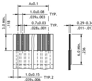
Accommodated FFC
