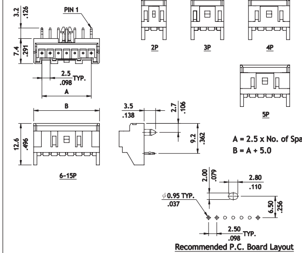
P/N CI60**P1HK0
