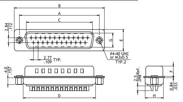
Plug Connector(C0/C1Type)
