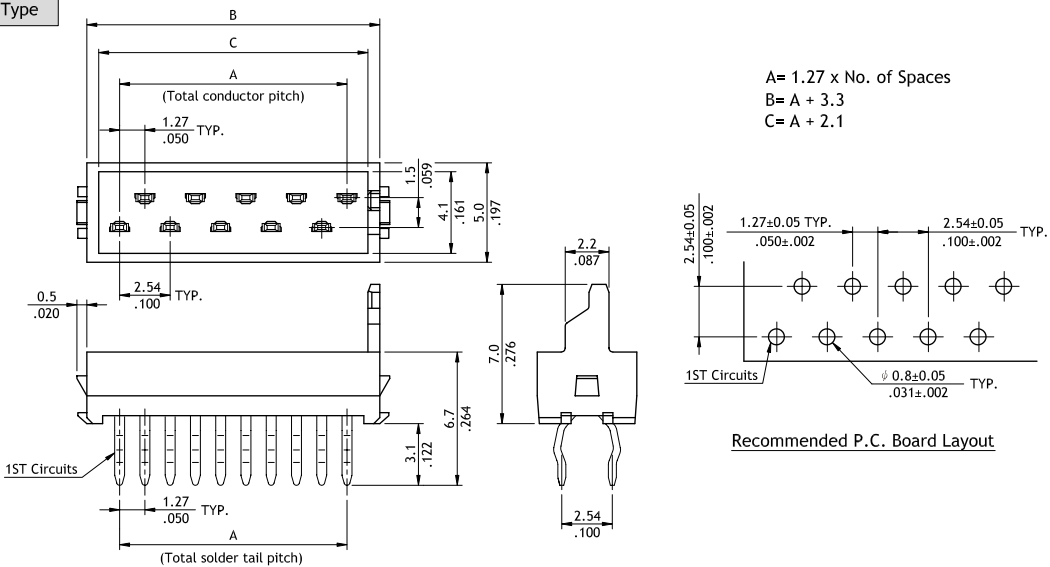
DIP Type
