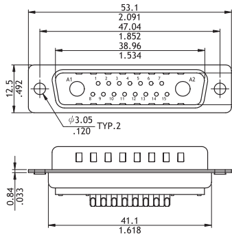
C8W8 (Plug Connector)
