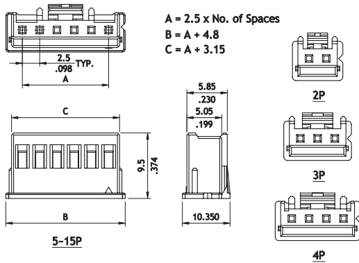
P/N CI60**P1VK0
