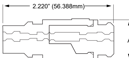
Mated Plug & Receptacle
